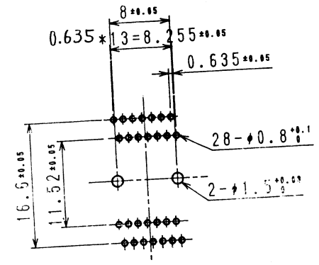
P.C.B. PATTERN (TOP VIEW)
